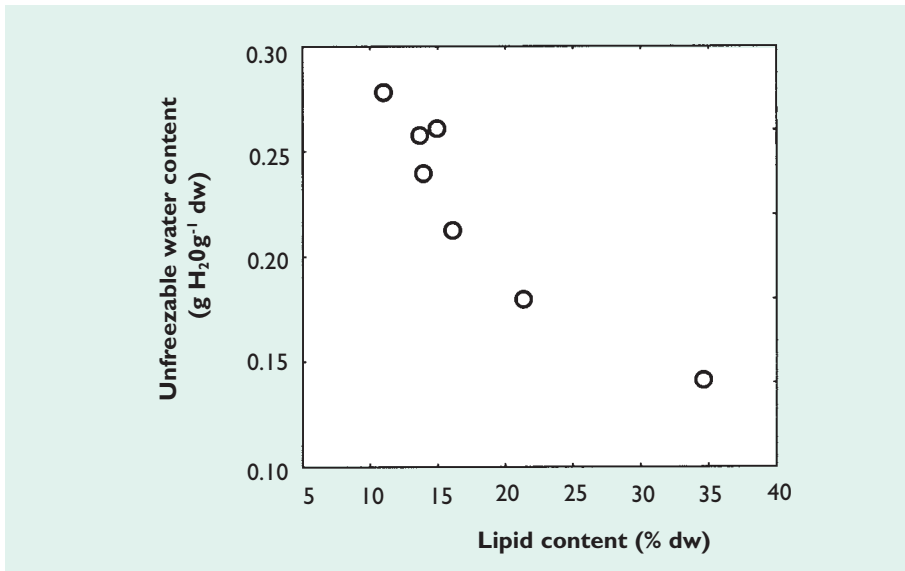
Figure 44.3 Relationship between the lipid content and the unfreezable water content, as determined from DSC analysis, of seeds of seven coffee species. (From Dussert et al. (2001), with permission of Blackwell Publishing).
